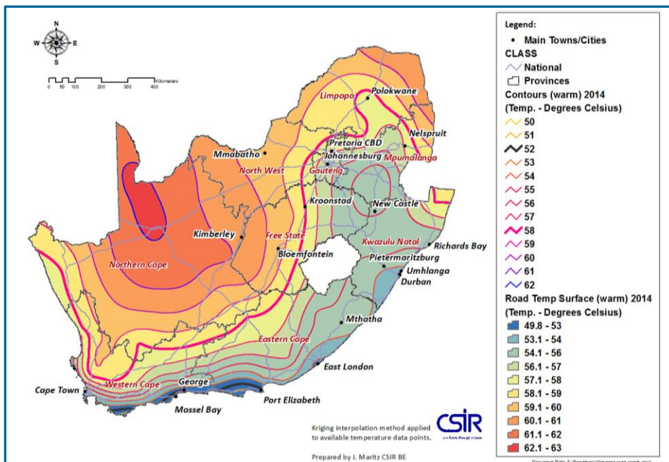
Figure 2: 7-day average maximum asphalt temperatures
