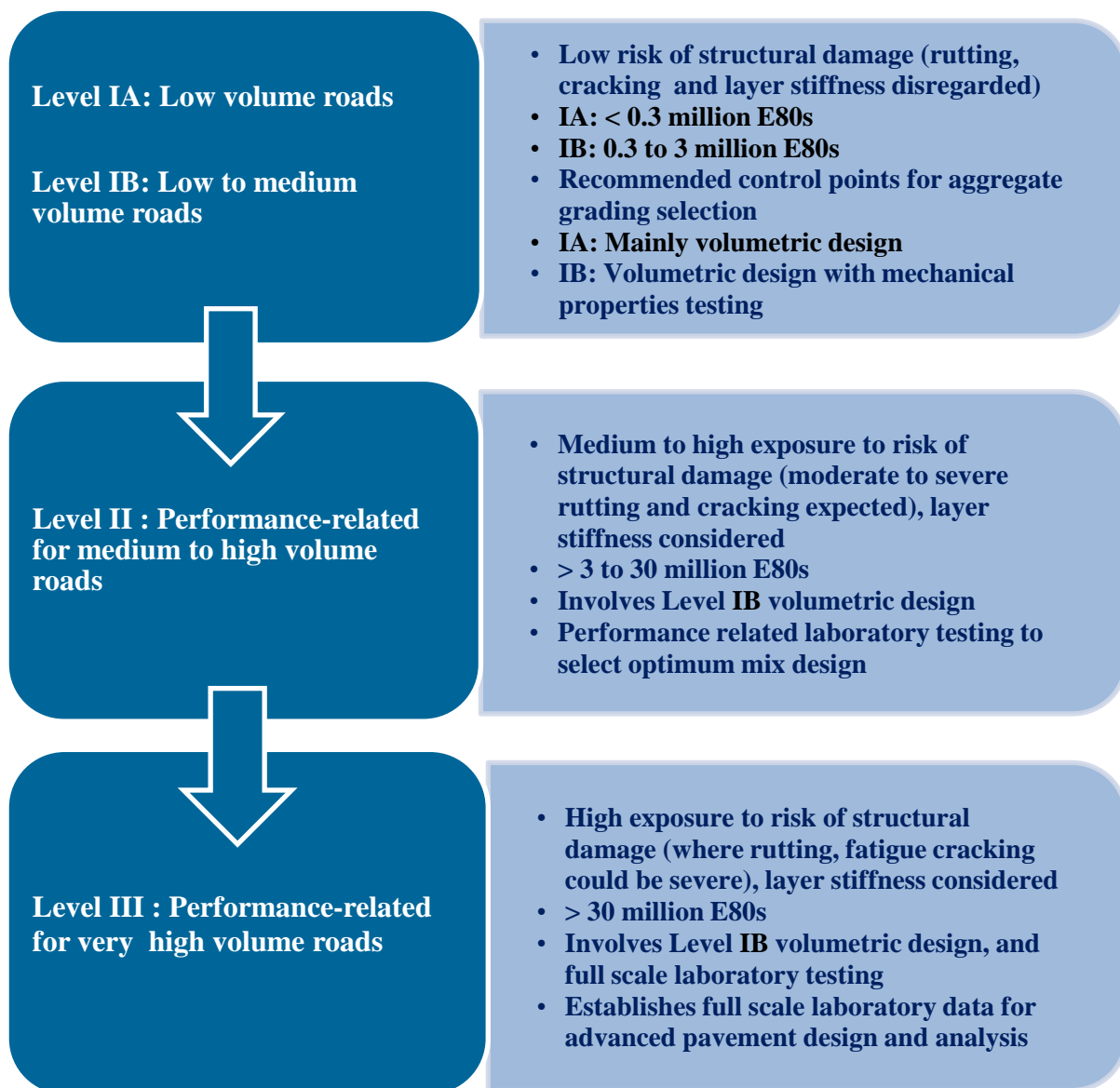
Figure 6: Mix design levels
