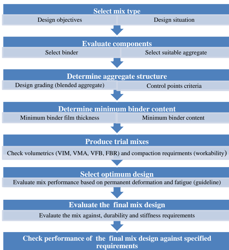
Figure 8: Level II and level III mix design process
