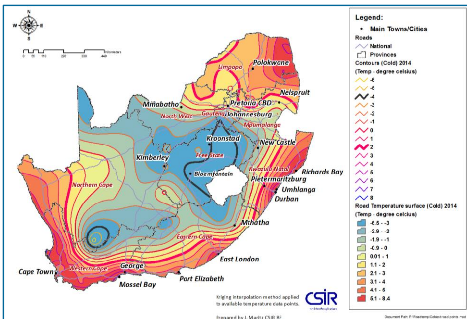
Figure 3: Minimum asphalt temperatures
