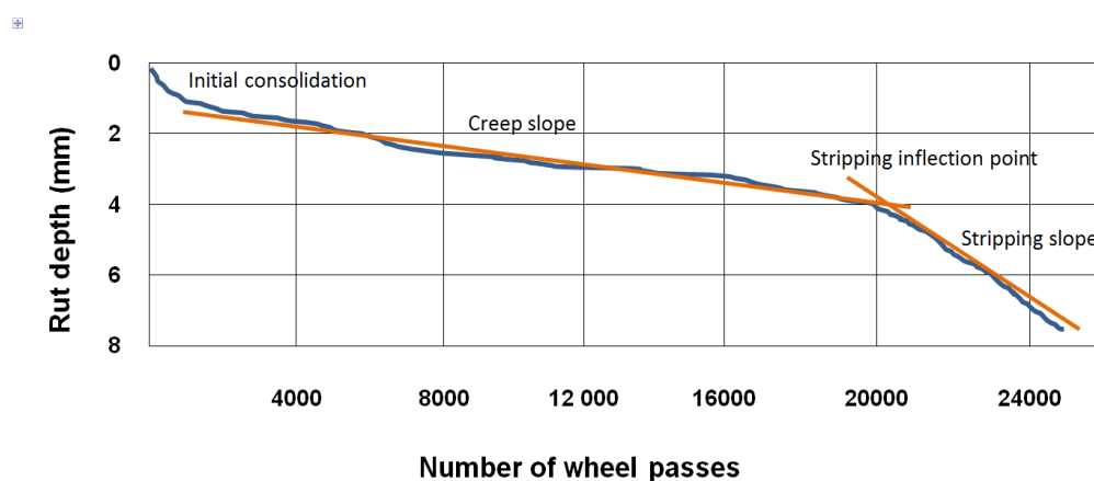
Figure 9: Definition of the Hamburg wheel tracking device results
