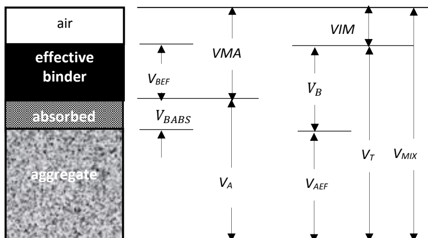
Figure 5: Volumetric parameters of compacted asphalt specimen
