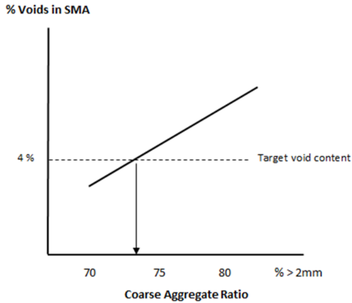
Figure B 3: Relationship of voids and coarse aggregate ratio
